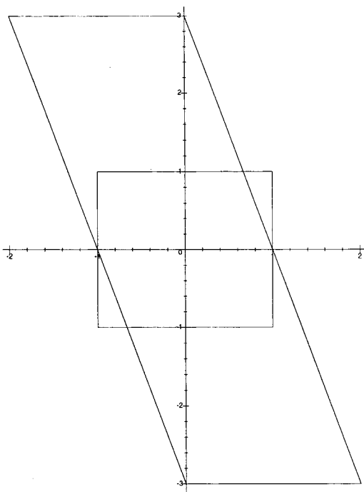
FIG. 3. First try for strict expansiveness.
